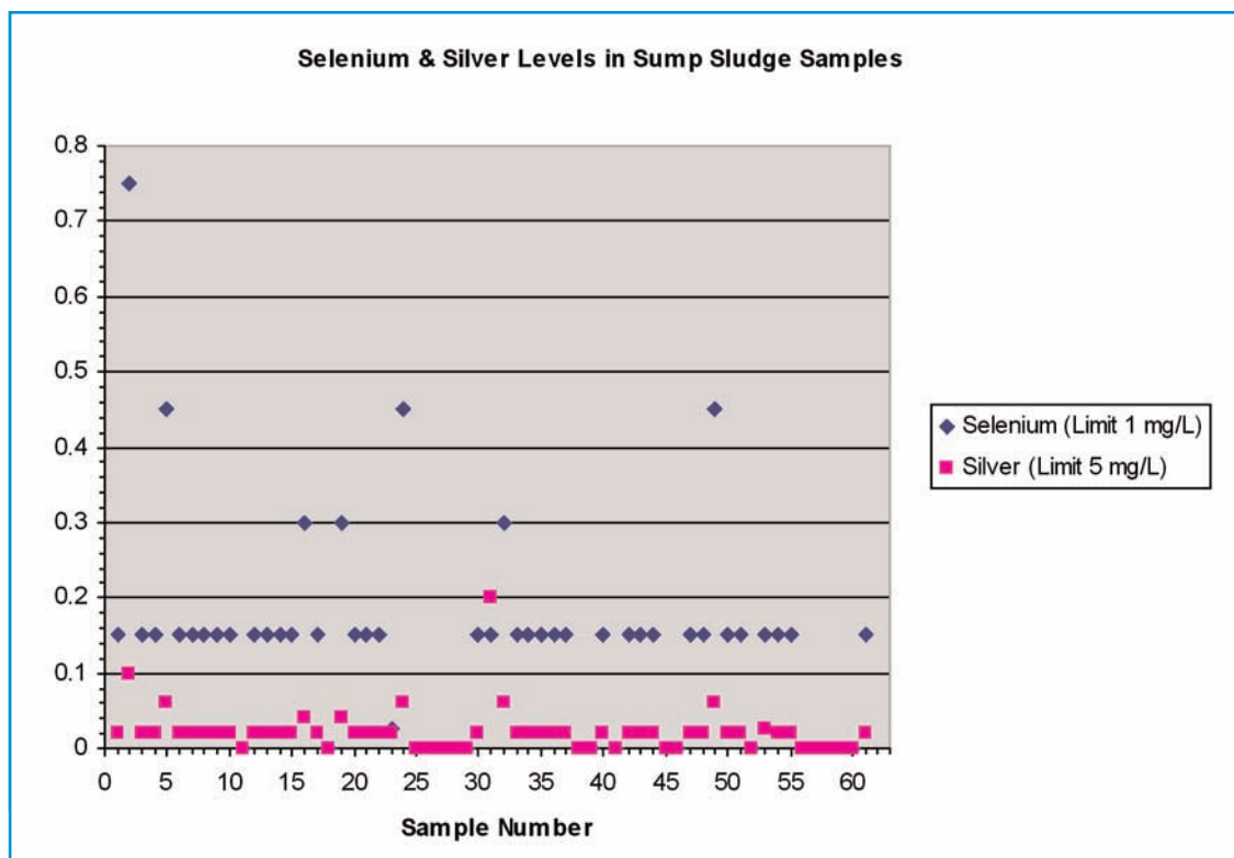
Figure 4. Selenium and Silver Concentrations in Sump Sludge Samples.
