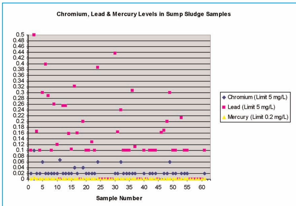
Figure 3. Chromium, Lead & Mercury Concentrations in Sump Sludge Samples.
