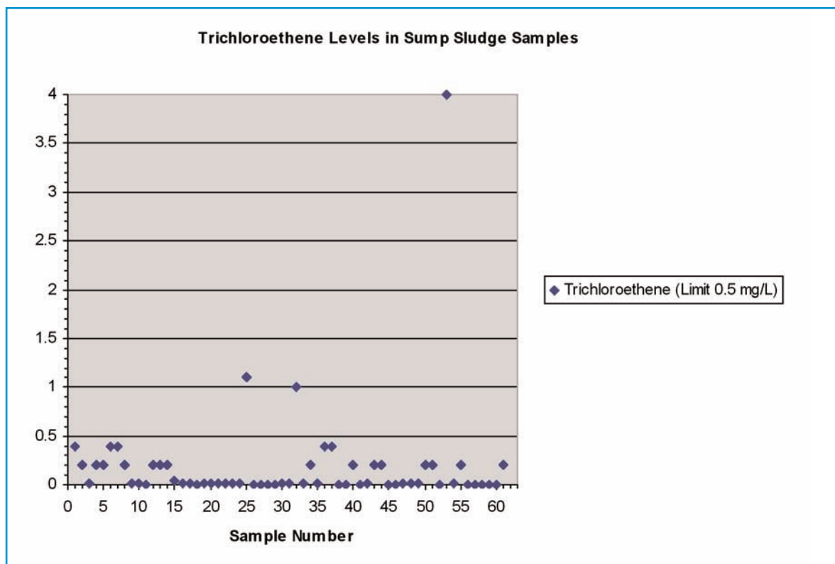
Figure 12. Trichloroethene Concentrations in Sump Sludge Samples.
