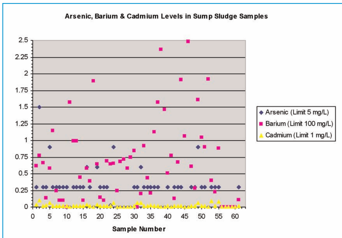
Figure 2. Arsenic, Barium & Cadmium Concentrations in Sump Sludge Samples.
