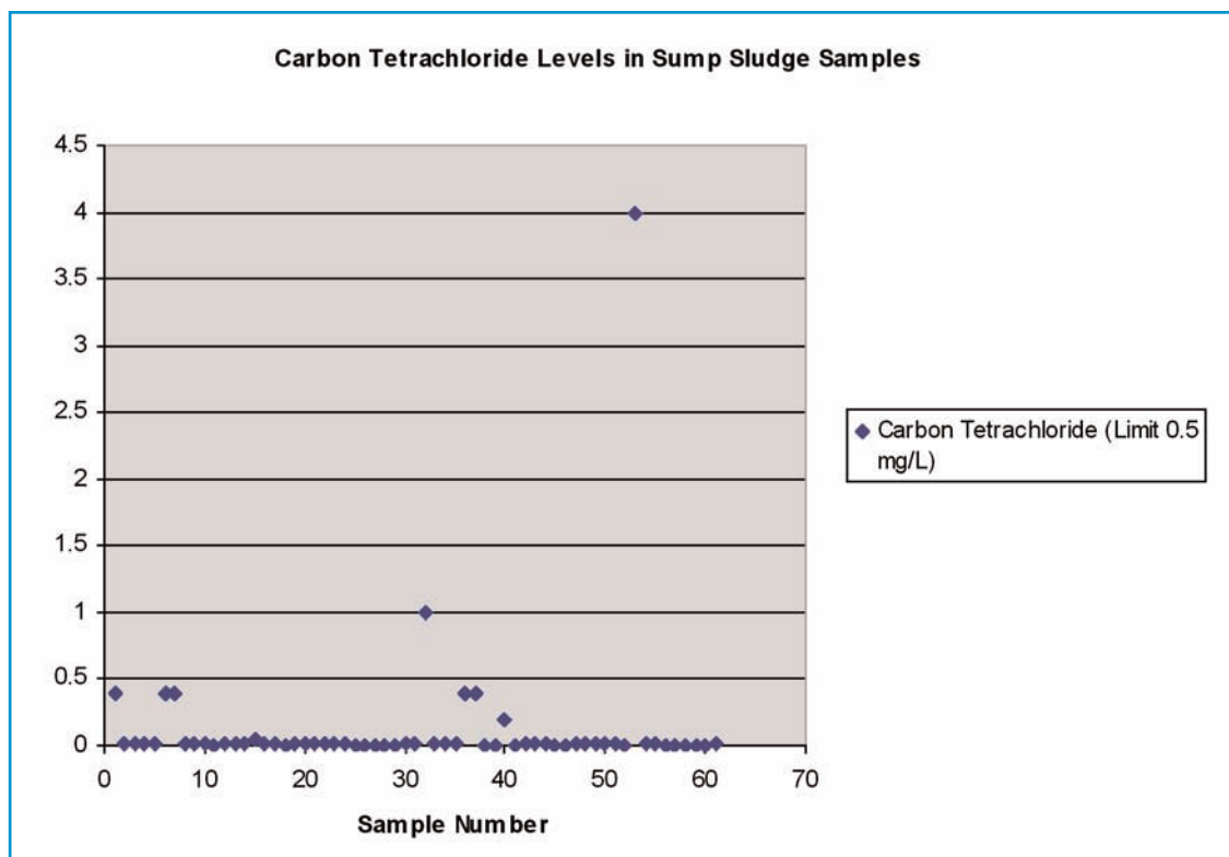
Figure 6. Carbon Tetrachloride Concentrations in Sump Sludge Samples.
