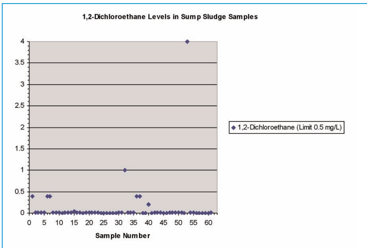
Figure 9. 1,2-Dichloroethane Concentrations in Sump Sludge Samples.
