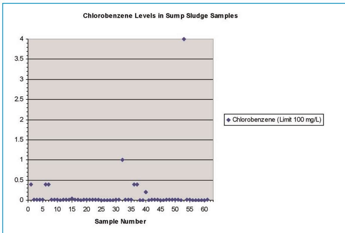
Figure 7. Chlorobenzene Concentrations in Sump Sludge Samples.
