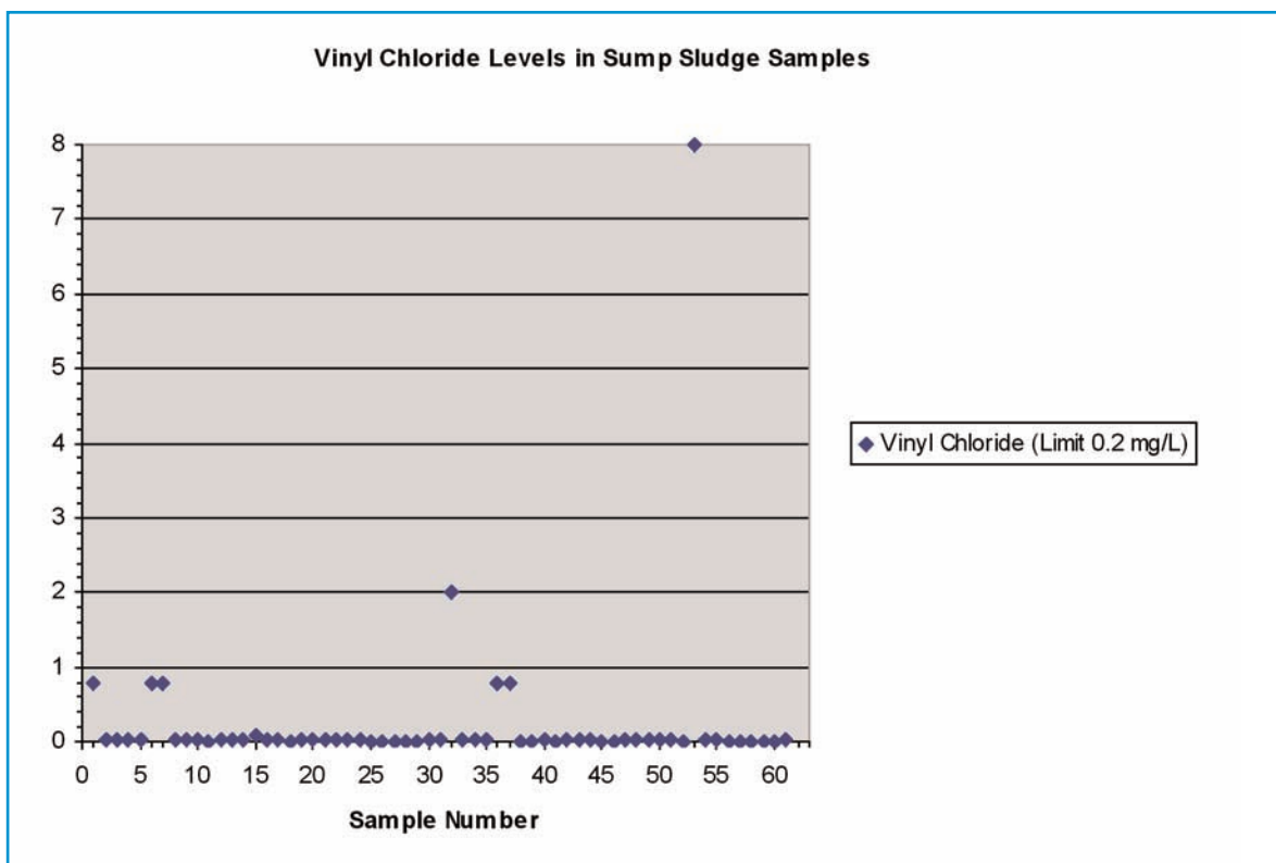
Figure 13. Vinyl Chloride Concentrations in Sump Sludge Samples.
