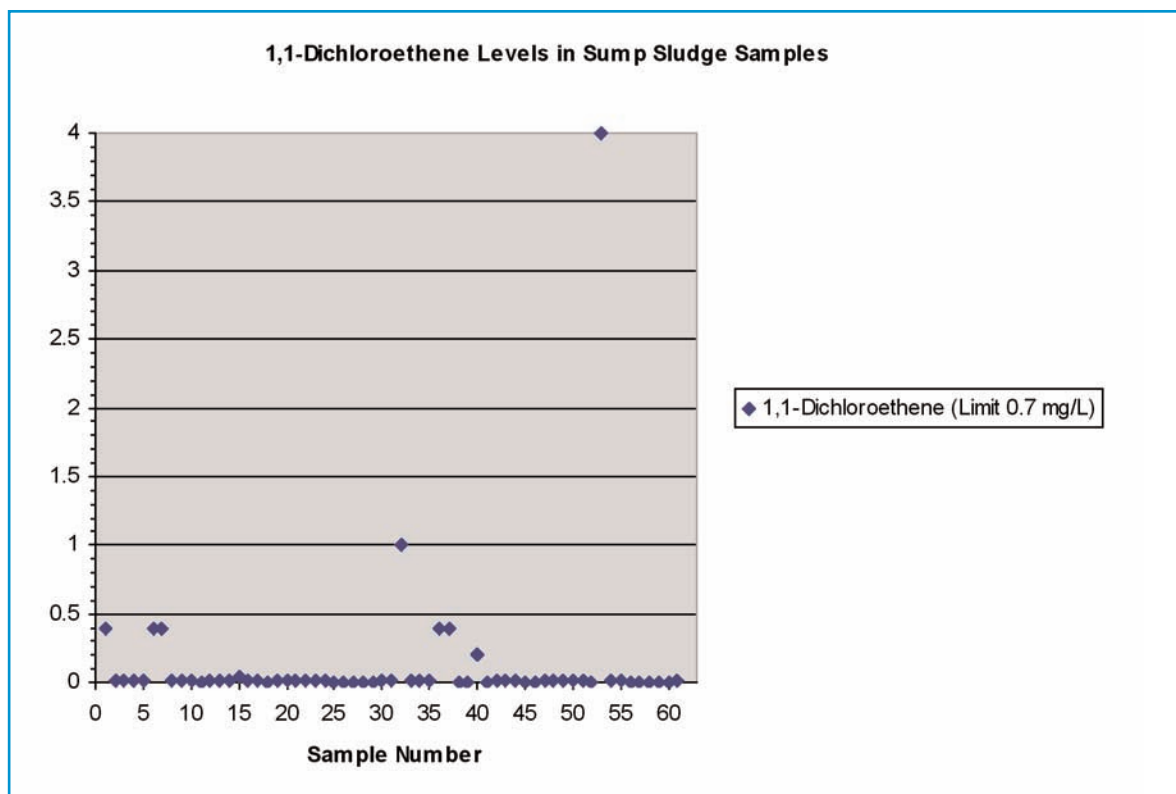
Figure 10. 1,1-Dichloroethene Concentrations in Sump Sludge Samples.
