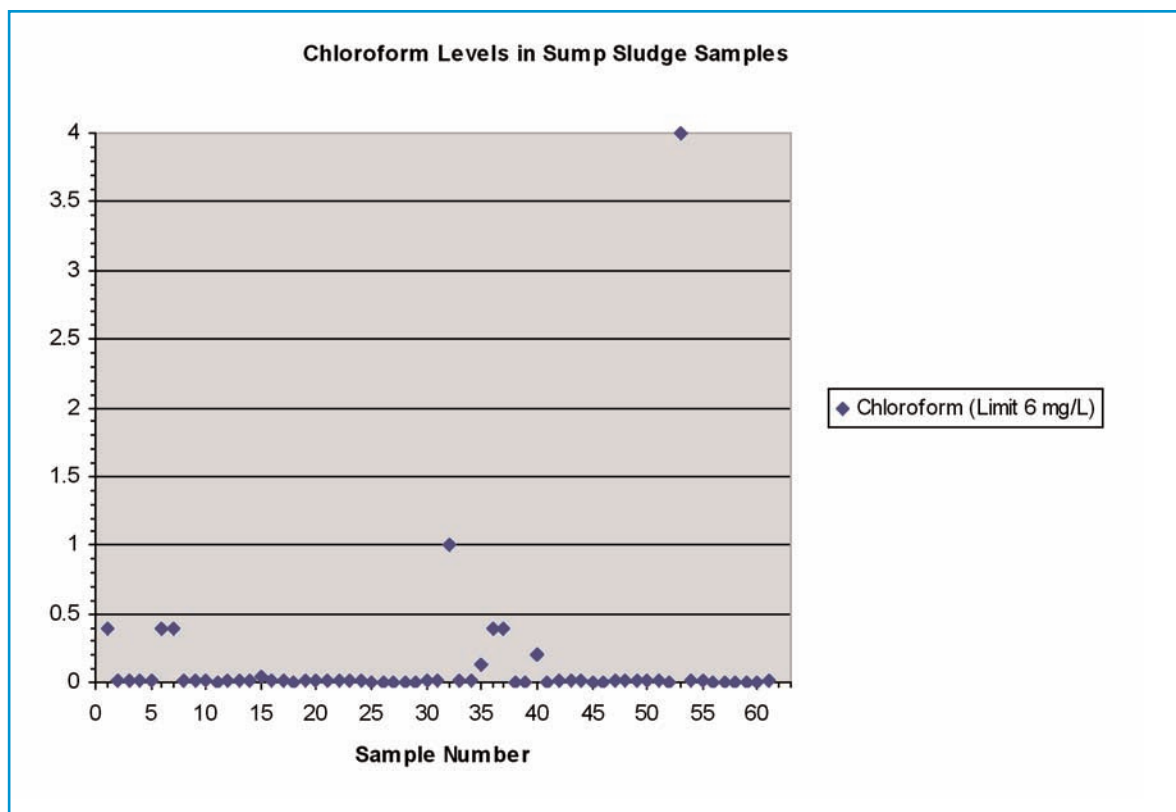
Figure 8. Chloroform Concentrations in Sump Sludge Samples.
