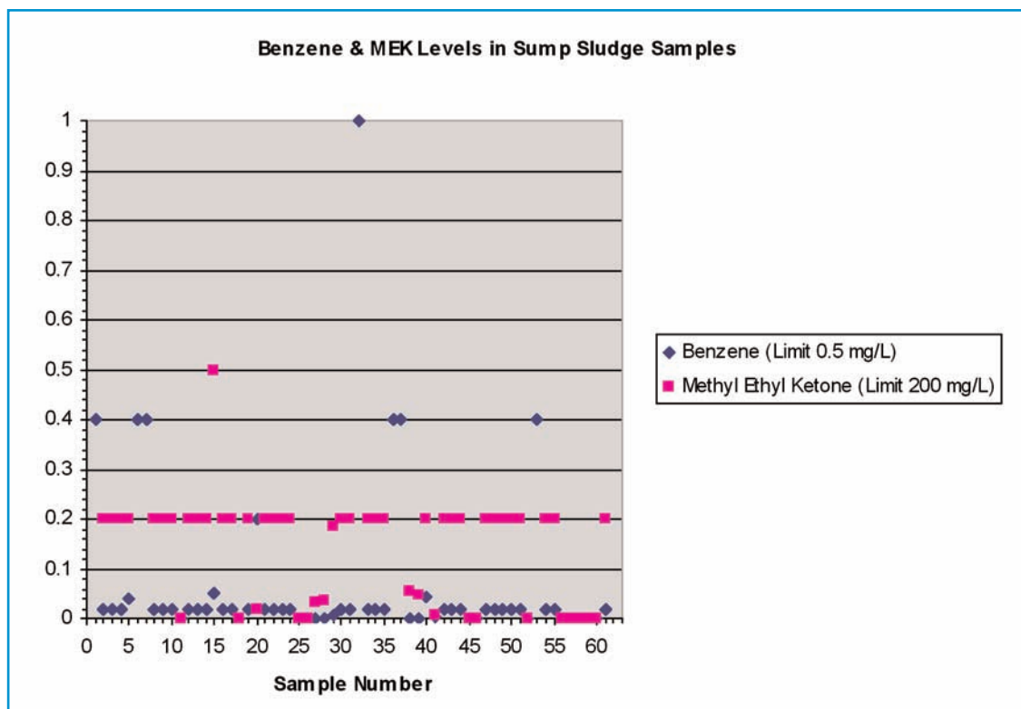
Figure 5. Benzene & Methyl Ethyl Ketone (MEK) Concentrations in Sump Sludge Samples.
