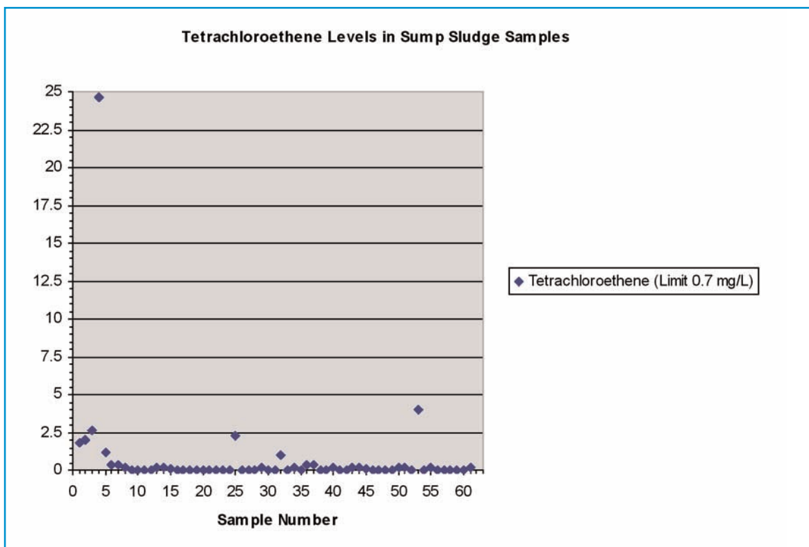
Figure 11. Tetrachloroethene Concentrations in Sump Sludge Samples.
